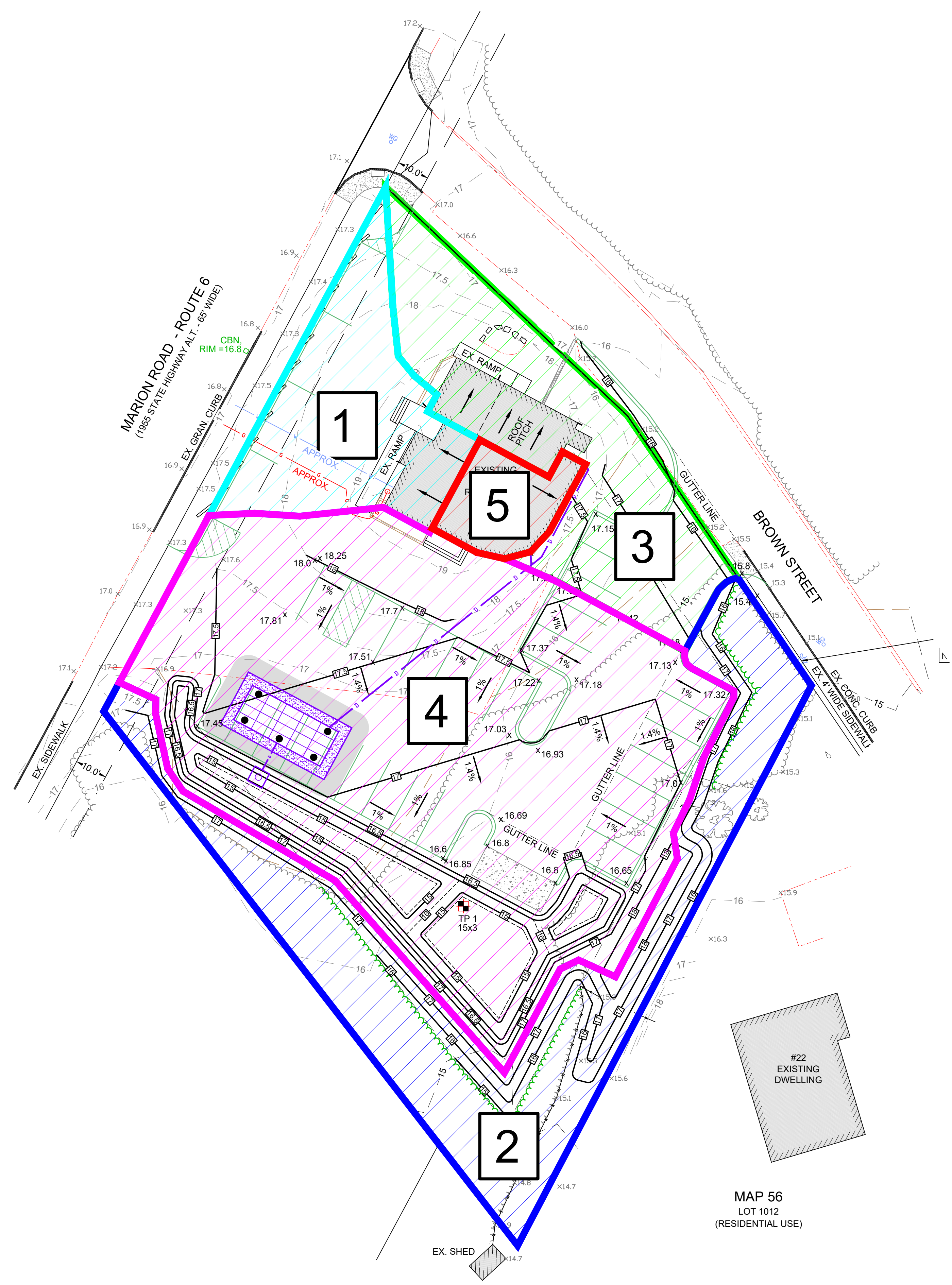
PROPOSED DRAINAGE AREAS SCALE: 1" = 20'
