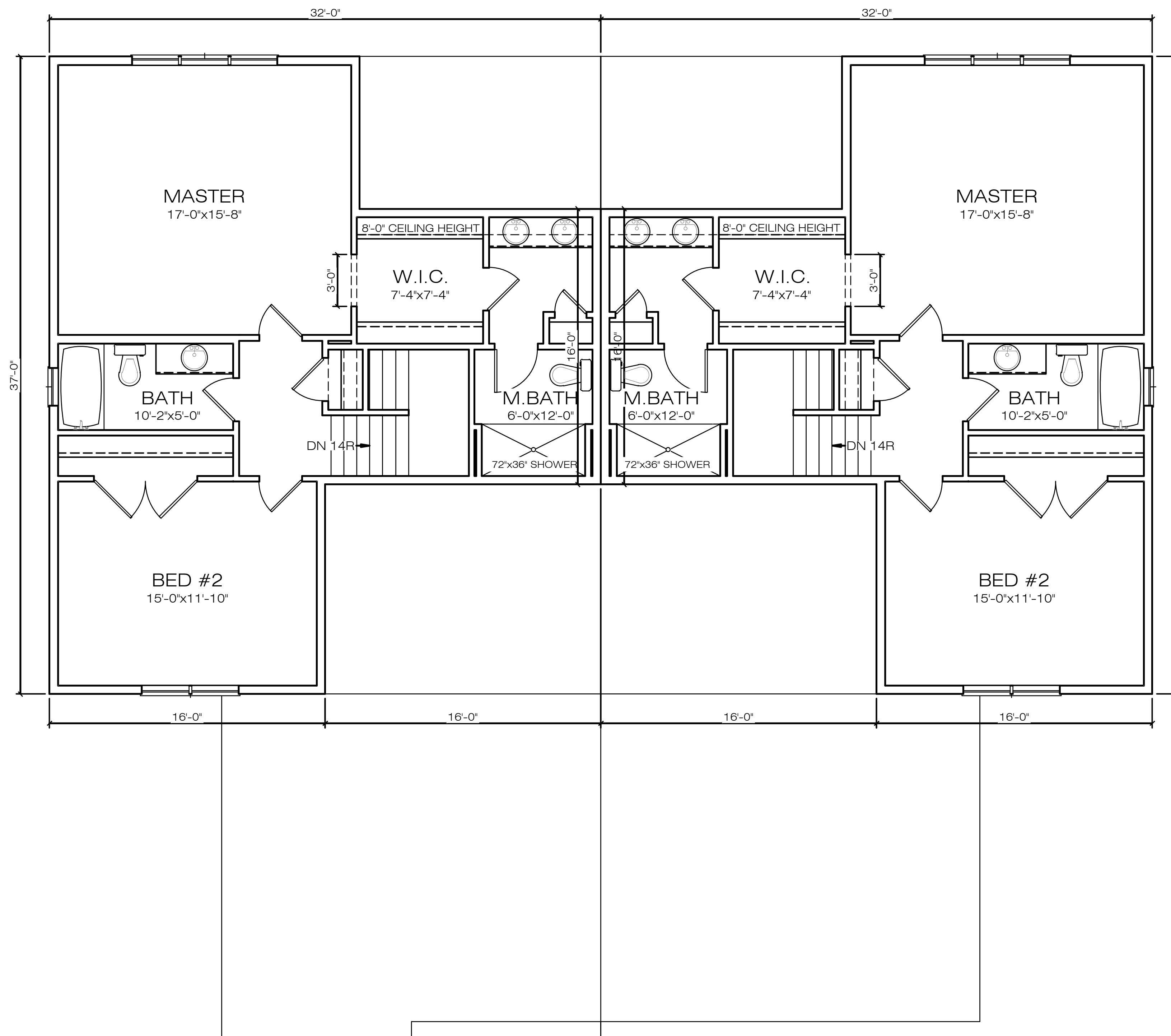
STANDISH SECOND FLOOR PLAN 8'-0" CEILING HEIGHT 870 SQ FT
