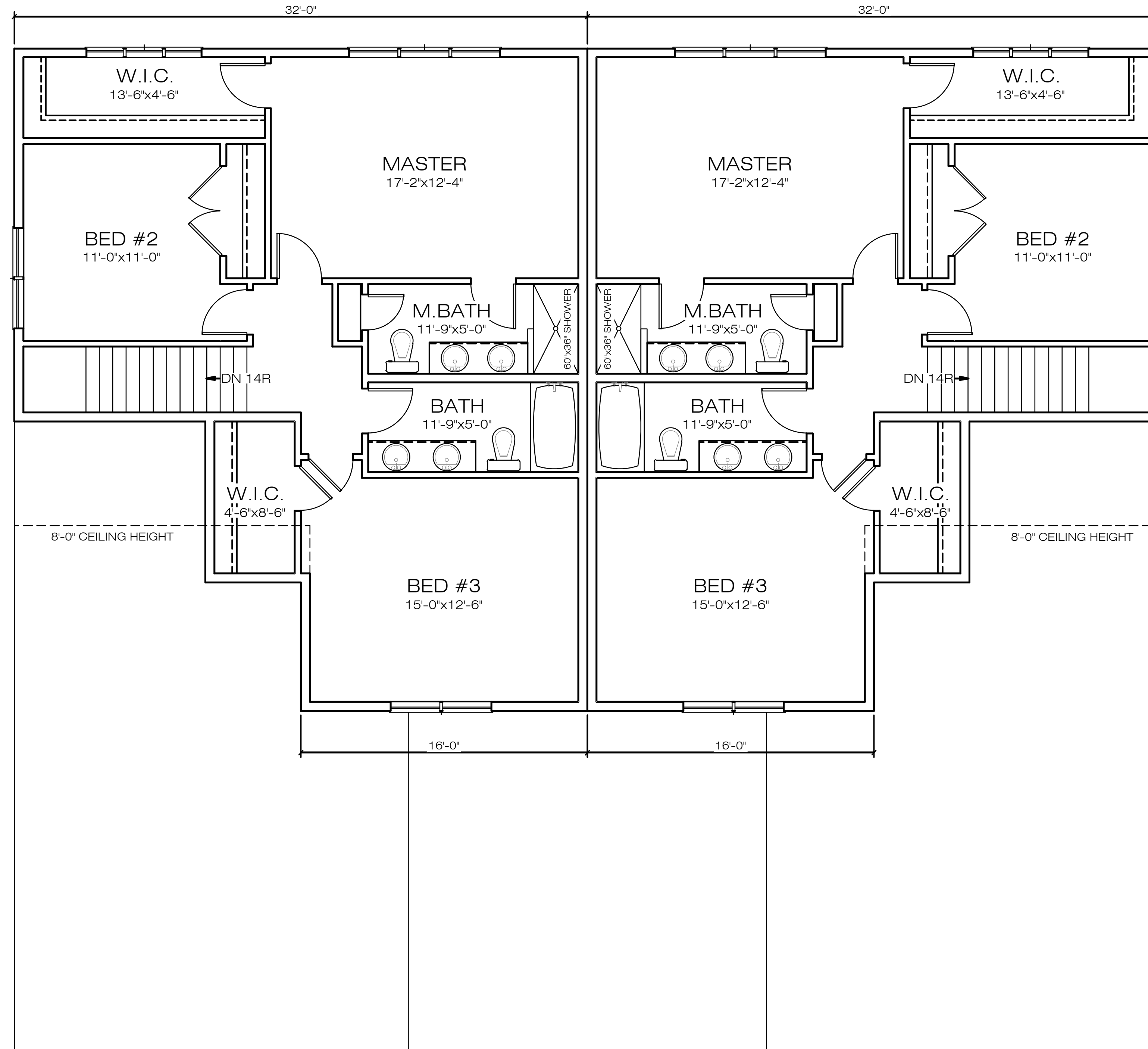
B STANDISH SECOND FLOOR PLAN 8'-0" CEILING HEIGHT 976 SQ FT
