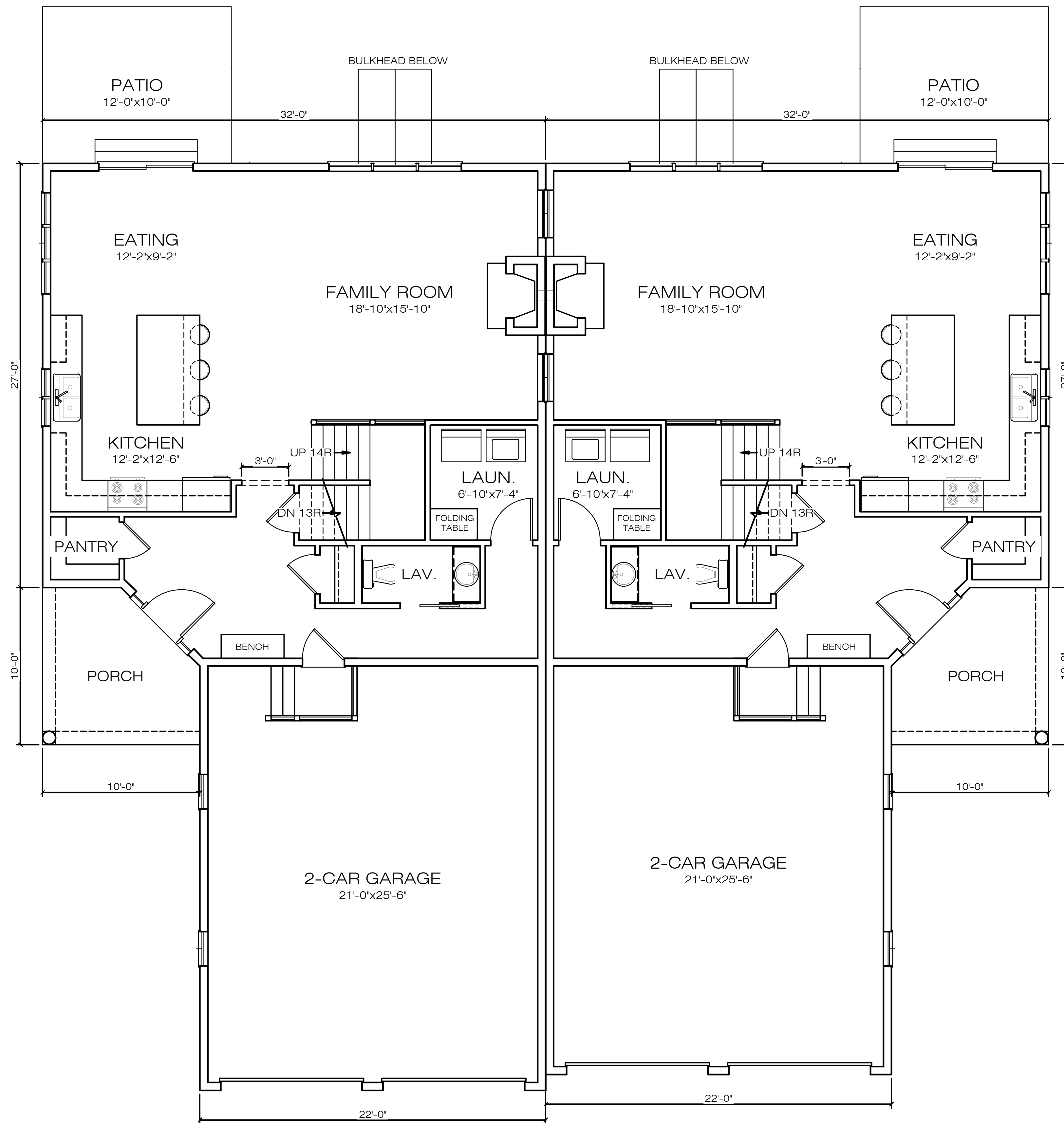
STANDISH FIRST FLOOR PLAN 8'-0" CEILING HEIGHT 987 SQ FT
