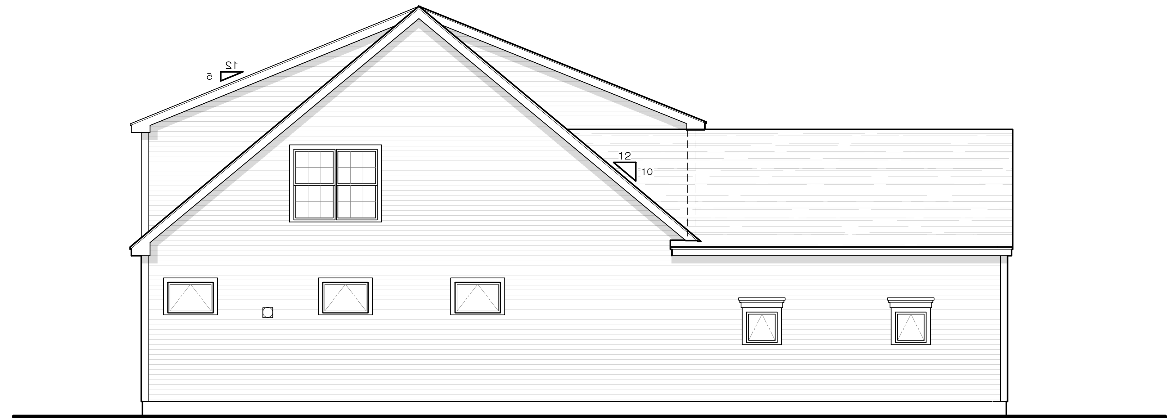
STANDISH LEFT ELEVATION
