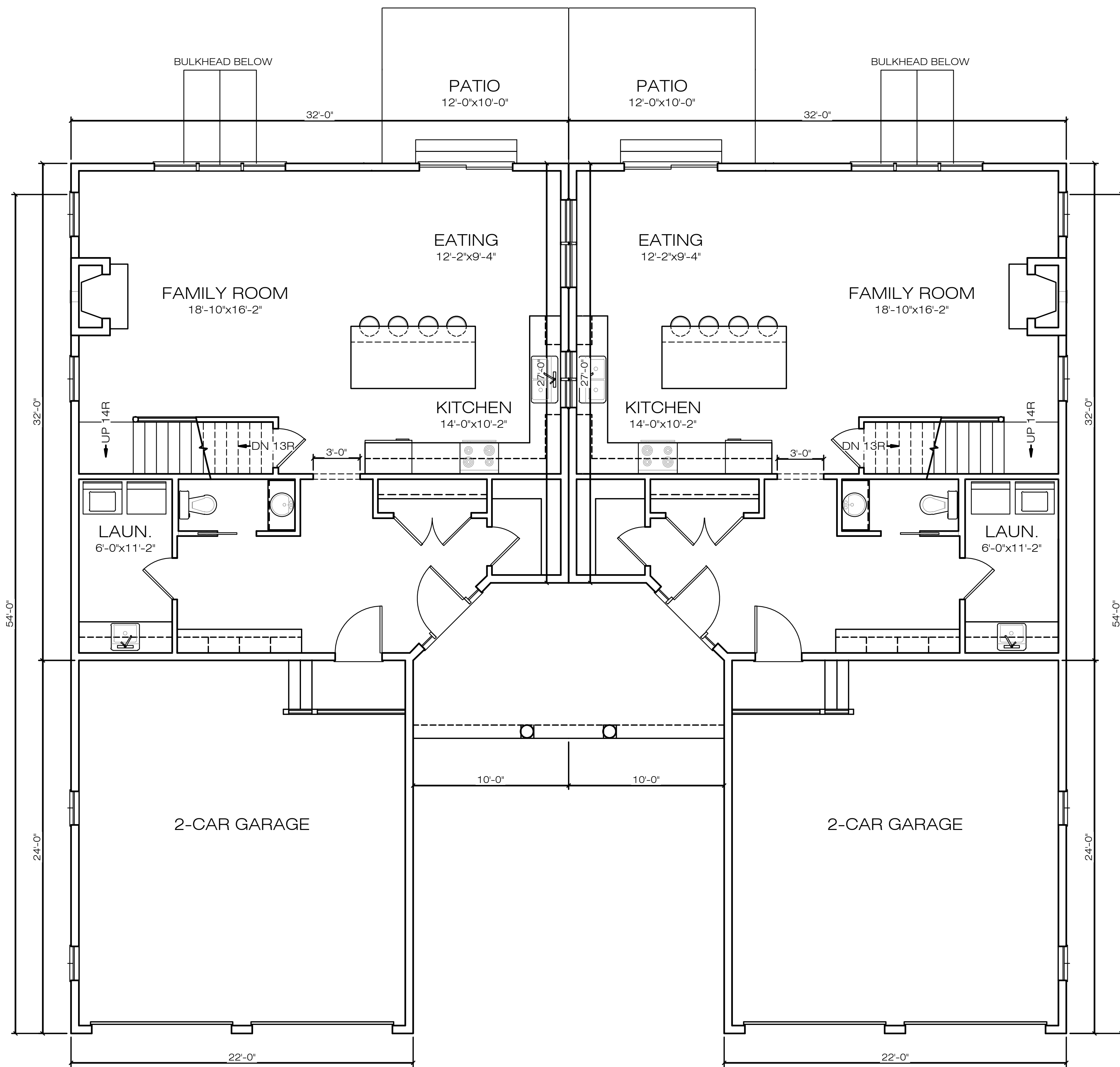
B STANDISH FIRST FLOOR PLAN 8'-0" CEILING HEIGHT 987 SQ FT
