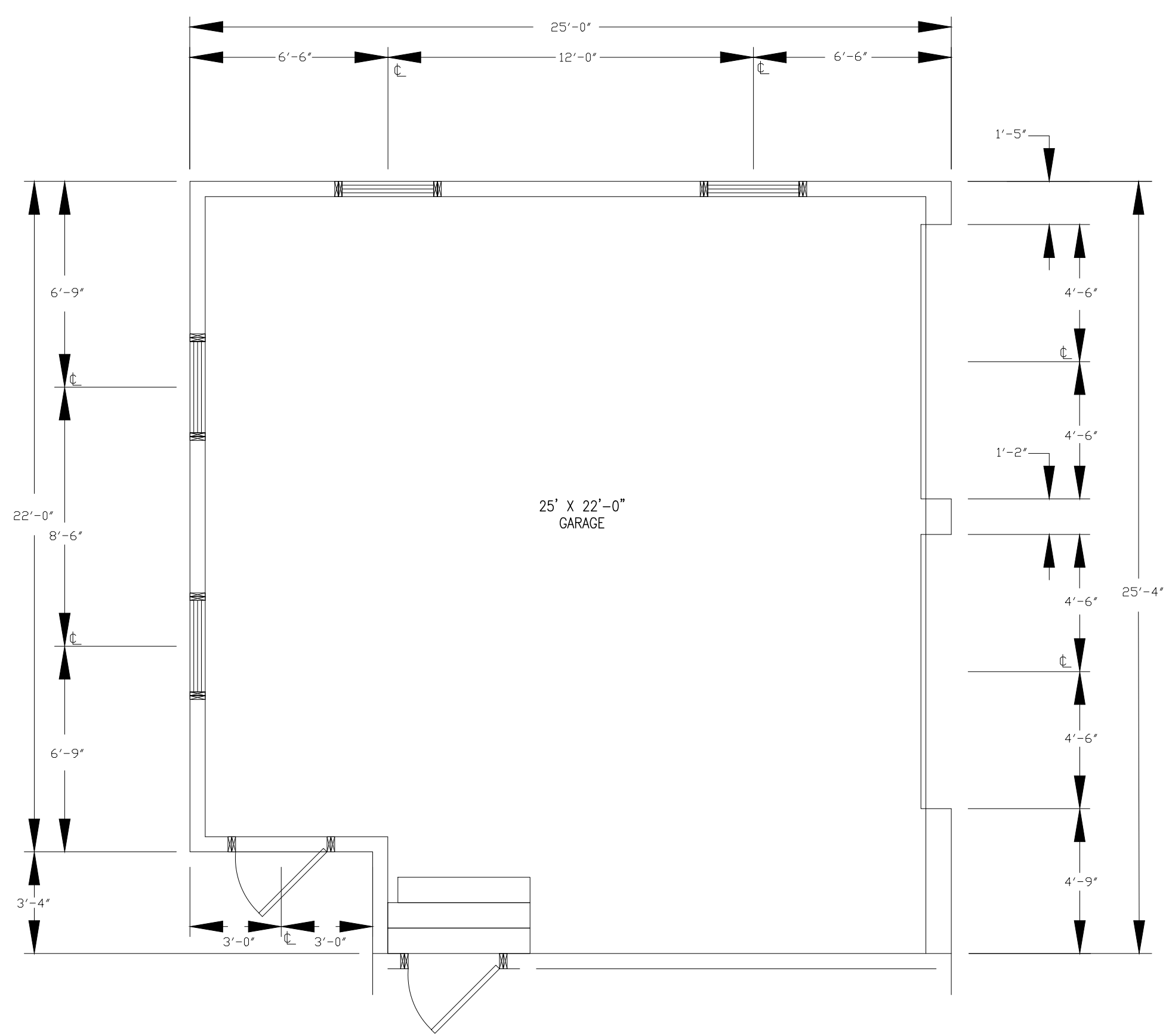
GARAGE LEVEL 1 DIMENSIONS
