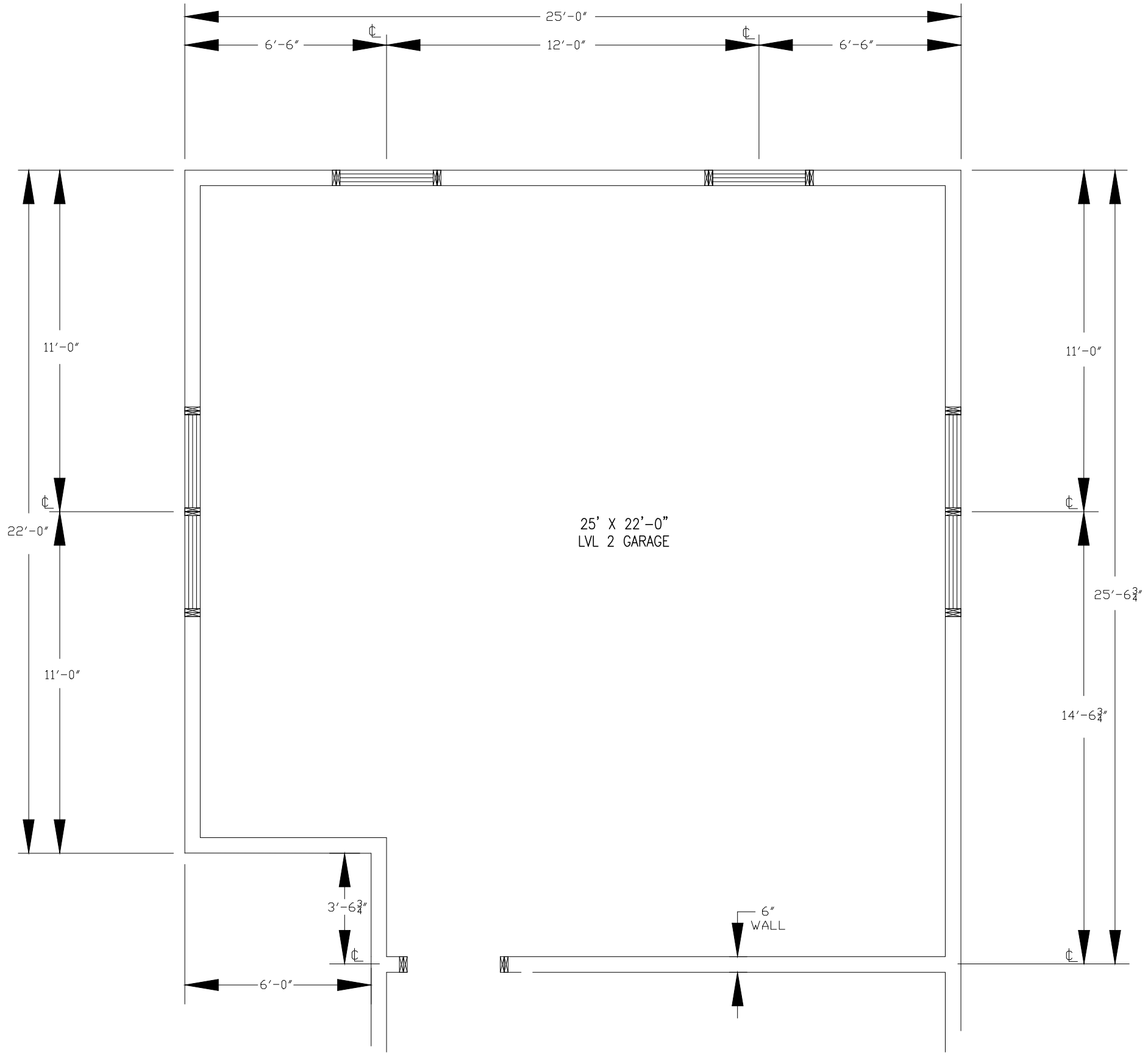
GARAGE LEVEL 2 DIMENSIONS
