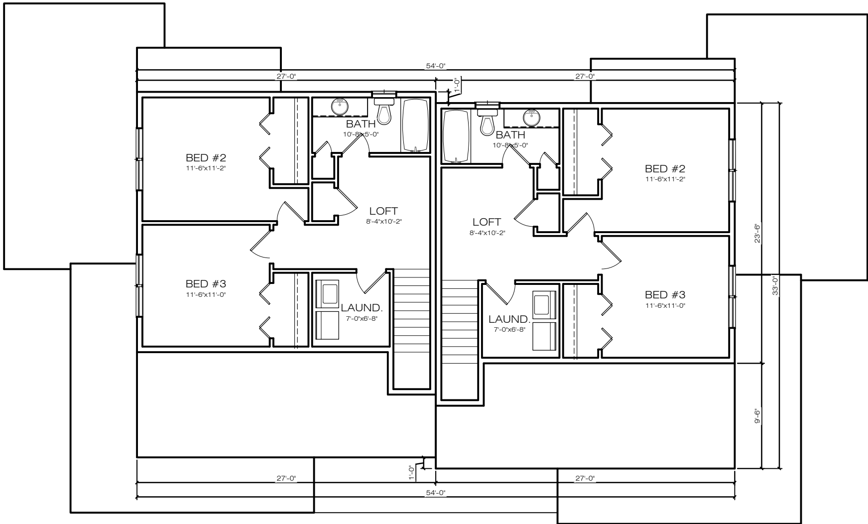
SECOND FLOOR PLAN 8 CEILING HEIGHT 633 SQ. FT.
