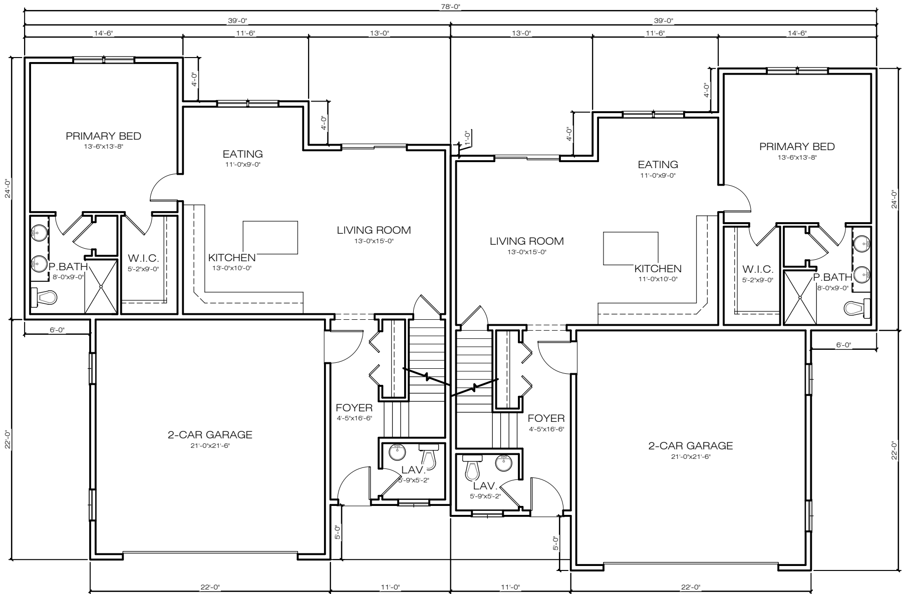
FIRST FLOOR PLAN 9' CEILING HEIGHT 1,018 SQ.FT.
