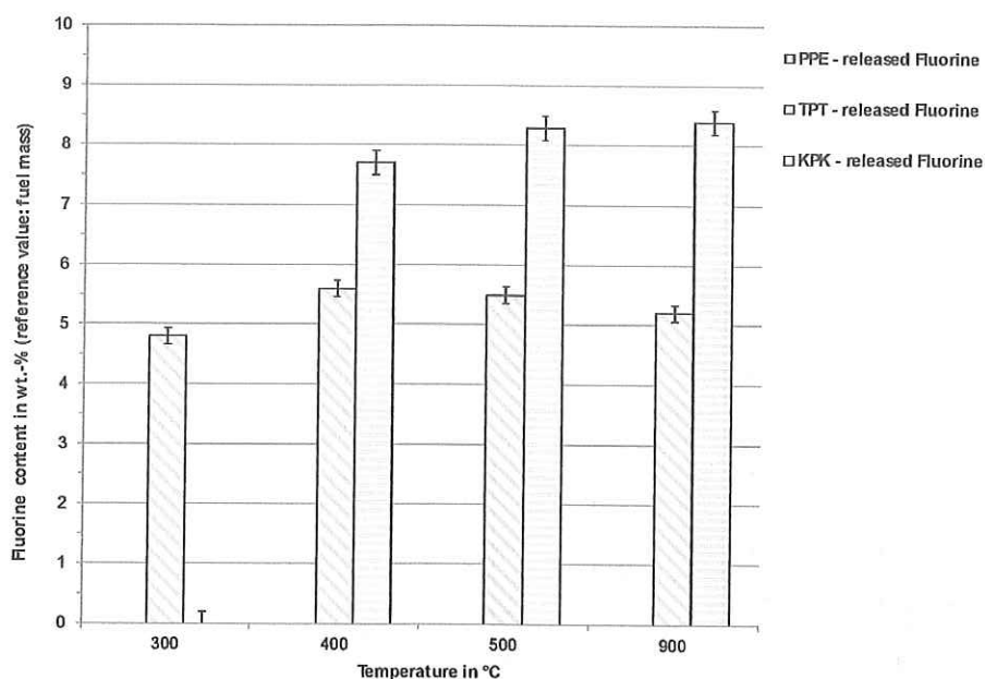
Figure 4. Pyrolysis results of fluorine transfer into the gas phase from PPE, TPT, and KPK.
